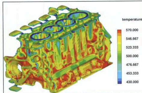
Fig 2. Temperature distribution after solidification
