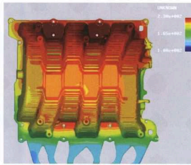
Fig 10. Simulation: of die temperature on the casting ISO surface
