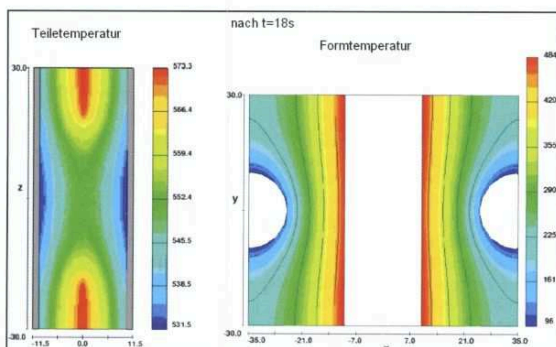
Fig 7. Influence of the casting temperature and of the die with a 20mm thick wall with cooling lines located 15mm from cavity
