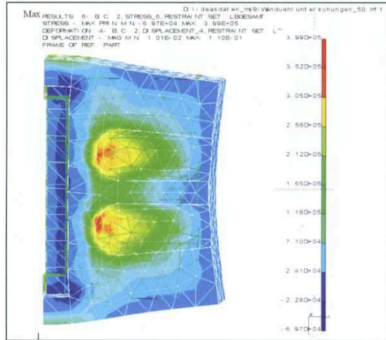
Fig 9. FEA calculation of thermal stress
